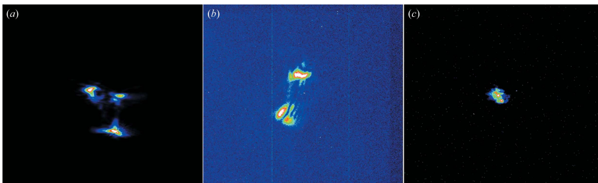
Figure 7 Coherent diffraction images for (a) (200)/(002) twin pair (PCMO1–18, frame 21; 2 s of exposure time, five accumulations, I_{\max} = 327670 counts s^{-1} ), (b) (220)/(022) twin pair (PCMO3–4, frame 33; 120 s of exposure time, one accumulation, I_{\max} = 2330 counts s^{-1} ) and (c) likely (200)/(002) twin pair (LPCMO16, frame 43; 60 s of exposure time, one accumulation, I_{\max} = 2440 counts s^{-1} ). Note the curved fringes that connect both twin peaks in (b). The full CCD recording area is shown for the sake of comparison.
