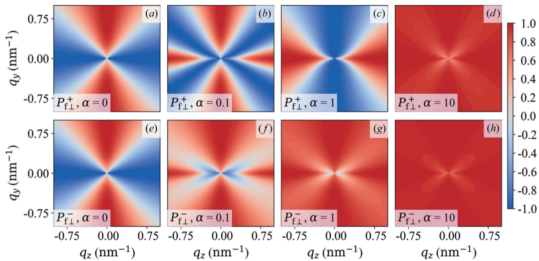
Figure 13 Plot of P_{f\perp}^+(q_y, q_z) (upper row) and P_{f\perp}^-(q_y, q_z) (lower row) for different values of \alpha = \text{constant} (see insets). A_H/A_M = 0.2 , \mu_0 H_i = 0.3 T, l_D = 0 .
