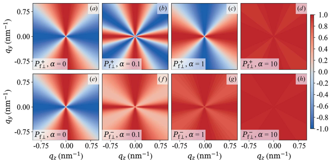
Figure 2 Plot of P_{f\perp}^+(q_y, q_z) (upper row) and P_{f\perp}^-(q_y, q_z) (lower row) in the saturated state for different values of \alpha (see insets) [equations (60a) and (60b)].
