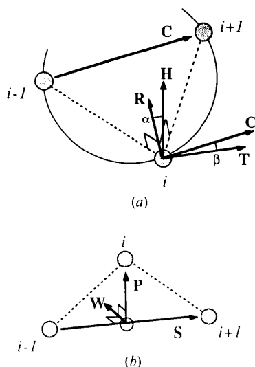
Fig. 3. (a) Construction of helix vectors for the atom Ca(i) . The vector C is the vector from atom Ca(i-1) to atom Ca(i+1) . Vector R is perpendicular to the plane formed by the atoms Ca(i-1) , Ca(i) and Ca(i+1) . Both C and R are normalized. The helix axis vector is then computed as H = (\cos\alpha)R + (\sin\alpha)C and the helix tangent vector as T = (\cos\beta)C - (\sin\beta)R . The constants \alpha = 32^\circ and \beta = 11^\circ were determined empirically and are optimized for a regular \alpha helix. Note that C and R are perpendicular but H and T are not. (b) The definition of vectors for atom Ca(i) used to create the \beta -strand arrow. The vector S is the strand-arrow direction vector for atom Ca(i) . The arrow normal vector P at atom Ca(i) is the vector from the midpoint between atoms Ca(i-1) and Ca(i+1) to atom Ca(i) . The vector W is used for creating the arrow planes and is simply perpendicular to S and P . Subsequent P vectors must not have an angle greater than 90^\circ between them, otherwise they are turned around.
