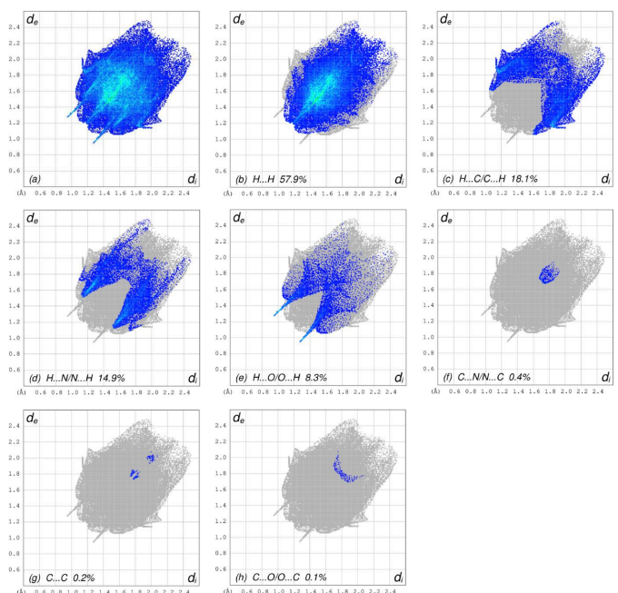
Figure 7 The full two-dimensional fingerprint plots for the title compound, showing (a) all interactions, and delineated into (b) H \cdots H, (c) H \cdots C/C \cdots H, (d) H \cdots N/N \cdots H (e) H \cdots O/O \cdots H, (f) C \cdots N/N \cdots C, (g) C \cdots C and (h) C \cdots O/O \cdots C interactions. The d_i and d_e values are the closest internal and external distances (in Å) from given points on the Hirshfeld surface.
