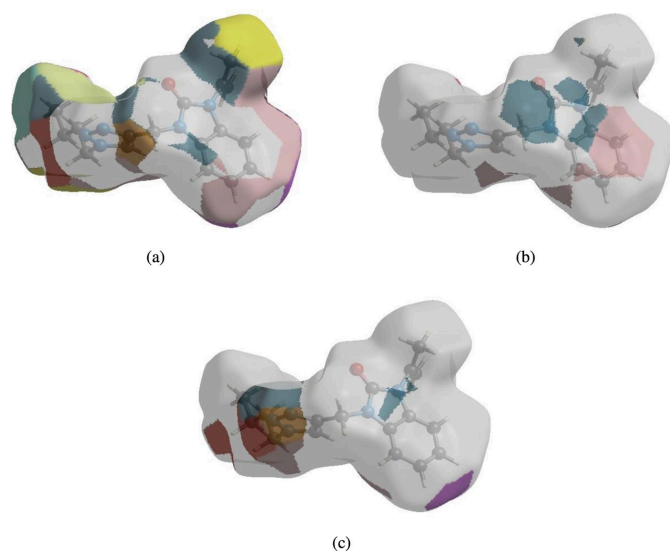
Figure 8 The HS representations with the function d_{\text{norm}} plotted onto the surface for (a) H \cdots H, (b) H \cdots C/C \cdots H and (c) H \cdots N/N \cdots H interactions.
