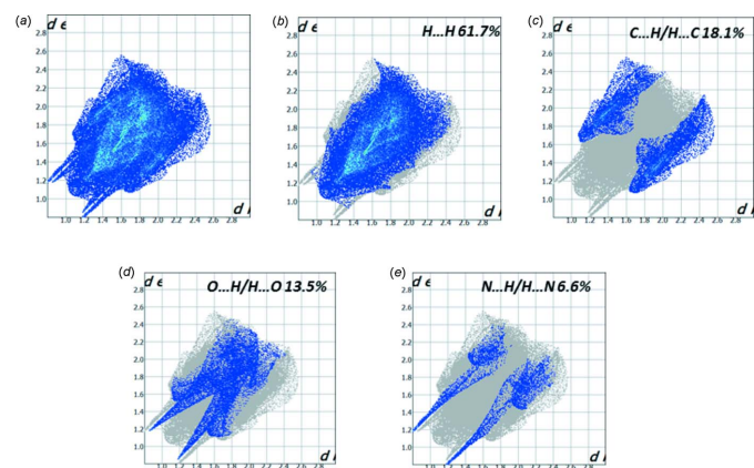
Figure 6 (a) The two-dimensional fingerprint plot for compound 4 , and those delineated into (b) \text{H}\cdots\text{H} (61.7%), (c) \text{C}\cdots\text{H}/\text{H}\cdots\text{C} (18.1%), (d) \text{O}\cdots\text{H}/\text{H}\cdots\text{O} (13.5%) and (e) \text{N}\cdots\text{H}/\text{H}\cdots\text{N} (6.6%) contacts.
