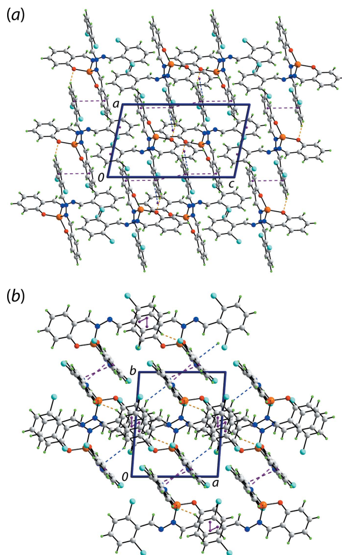
Figure 3 Molecular packing in the crystal of (I): (a) supramolecular layer sustained by C-H\cdots O , C-H\cdots \pi and \pi - \pi interactions shown as orange, blue and purple dashed lines, respectively, and (b) a view of the unit-cell contents in a projection down the c axis.
