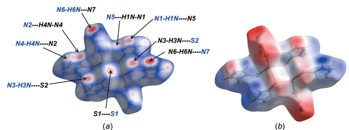
Figure 4 A view of the Hirshfeld surface for (I) mapped over (a) d_{\text{norm}} and (b) the electrostatic potential; the red and blue regions represent negative and positive electrostatic potentials, respectively.
