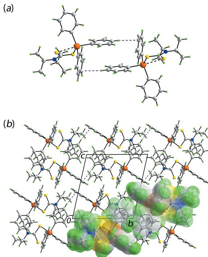
Figure 2 Molecular packing in the crystal of (I): (a) supramolecular dimer sustained by localized phenyl-C—H···C(phenyl) interactions shown as purple dashed lines and (b) a view of the unit-cell contents in projection down the a axis. One column of dimeric aggregates is highlighted in space-filling mode.
