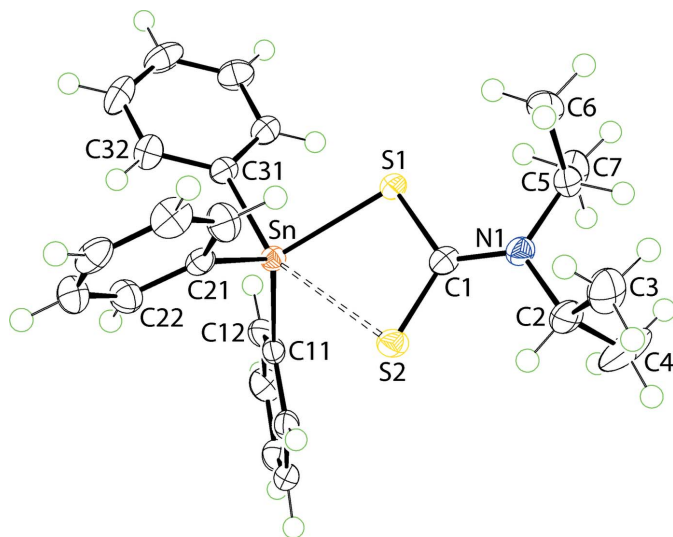
Figure 1 The molecular structure of (I) showing the atom-labelling scheme and displacement ellipsoids at the 70% probability level. The long Sn···S2 contact is indicated by a double-dashed line.
