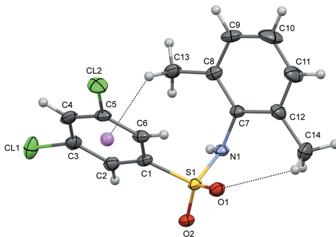
Figure 2 The molecular structure of (II) with displacement ellipsoids drawn at the 50% probability level. Intramolecular C–H···O and C–H··· \pi hydrogen interactions are shown as dotted lines.
