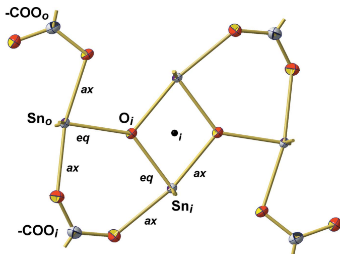
Figure 3 Location of axial ( ax ) and equatorial ( eq ) bonds with respect to the trigonal-bipyramidal coordination at the inner ( \text{Sn}_i ) and outer ( \text{Sn}_o ) Sn atoms and of the outer ( -\text{COO}_o ) \mu_1 - and inner ( -\text{COO}_i ) \mu_2 -carboxylate groups.
