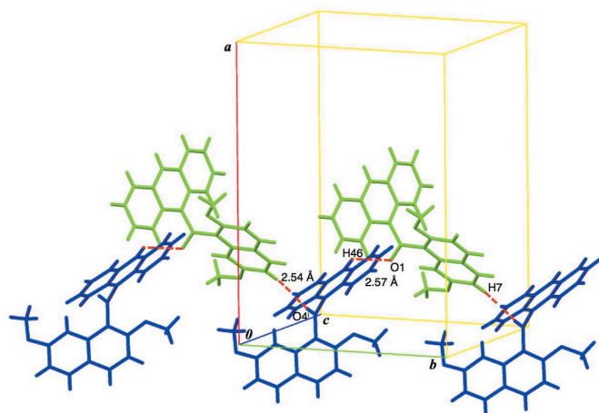
Figure 4 Two kinds of ( sp^2 )C–H...O=C hydrogen bonds between conformers A and B are shown as red broken lines. [Symmetry code: (i) x, y - 1, z .]
