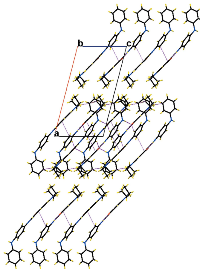
Figure 3 A view along the c axis of the crystal packing of the title compound. The hydrogen bonds, C–H··· \pi interactions and \pi – \pi interactions between the benzene ring and the imino group are shown as dashed lines (see Table 1 for details; for the latter interactions, the atoms involved are shown).
