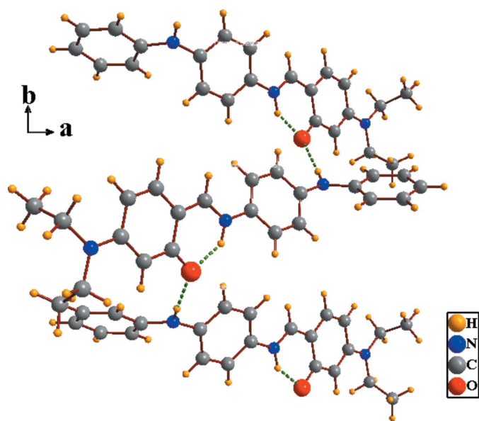
Figure 2 A view of the one-dimensional -A-B-A-B- zigzag hydrogen-bonded chain extending along the b axis. Hydrogen bonds are shown as dashed lines; see Table 1 for details.
