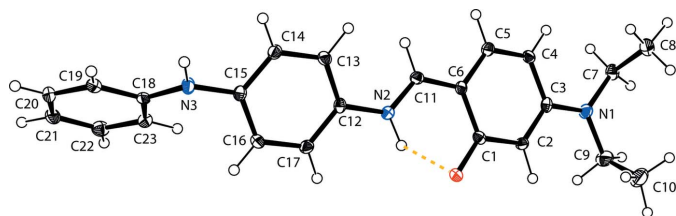
Figure 1 The molecular structure of the title compound, showing the atom labelling and the intramolecular N–H···O hydrogen bond as a dashed line (see Table 1 for details). Displacement ellipsoids are drawn at the 40% probability level.
