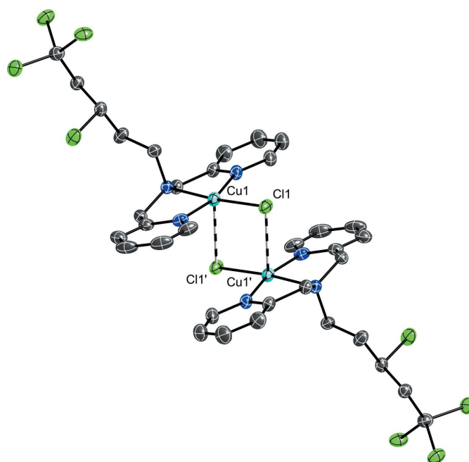
Figure 2 Dimer interactions between two [Cu(C 17 H 19 N 3 Cl 4 )(Cl)] ( 1 ) molecules, shown with 50% probability ellipsoids for the primary orientations of the disordered sites. H atoms are removed for clarity. The symmetry operation to generate the additional cation is 1 - x, 1 - y, 1 - z .
