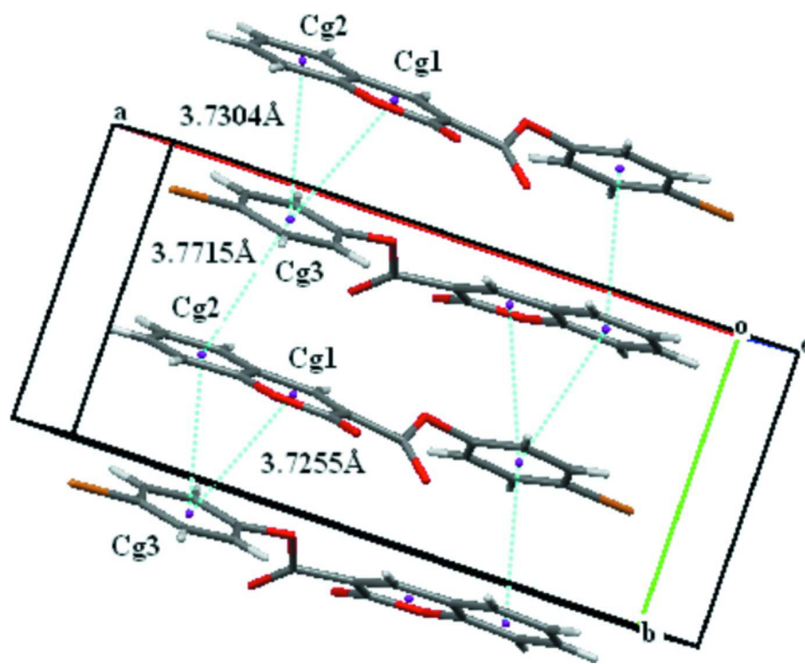
Figure 3 Various \pi - \pi interactions observed in the crystal packing
