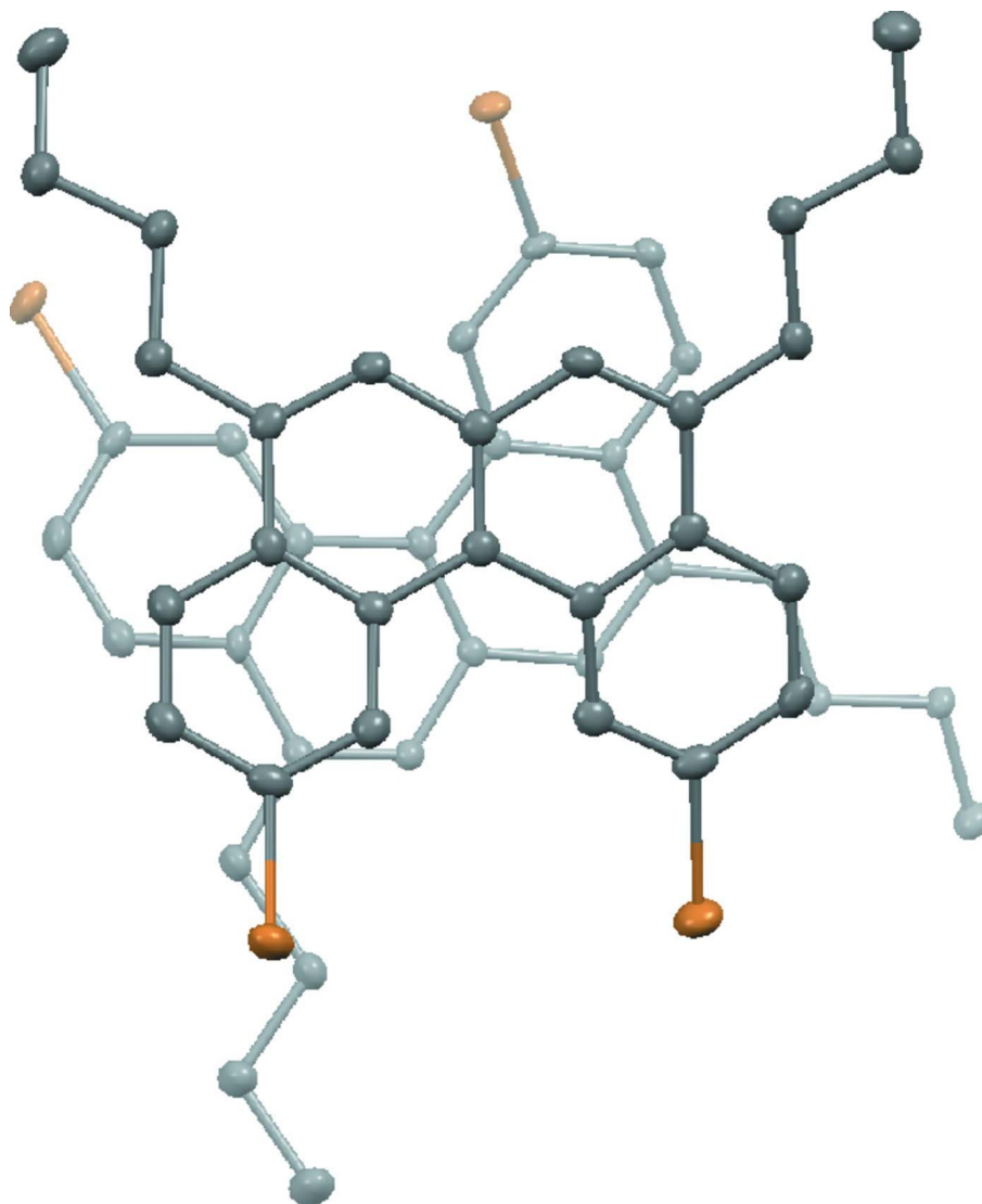
Figure 3 Stacking structure of the ( P )-form. Hydrogen atoms are omitted for clarity.
