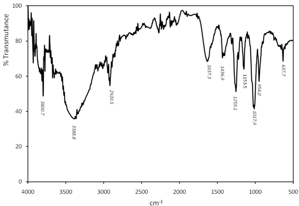
Figure 3 IR spectrum of the title compound (solid state, RT).
