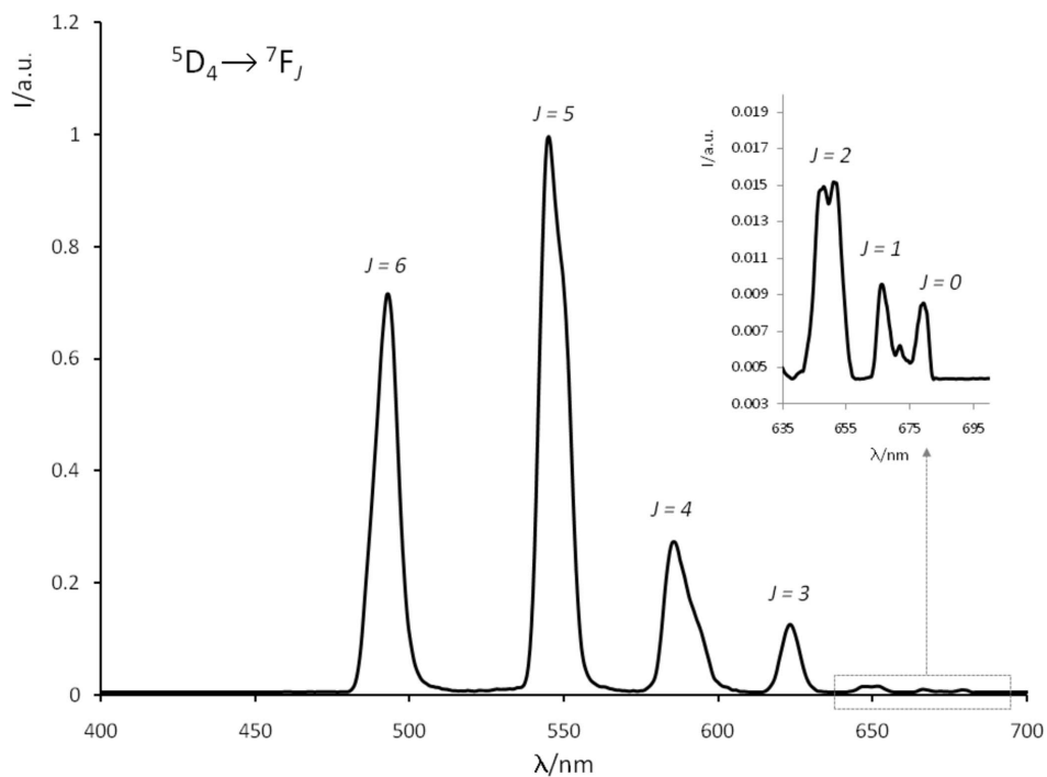
Figure 2 Phosphorescence spectrum of the title compound (solid state, RT).
