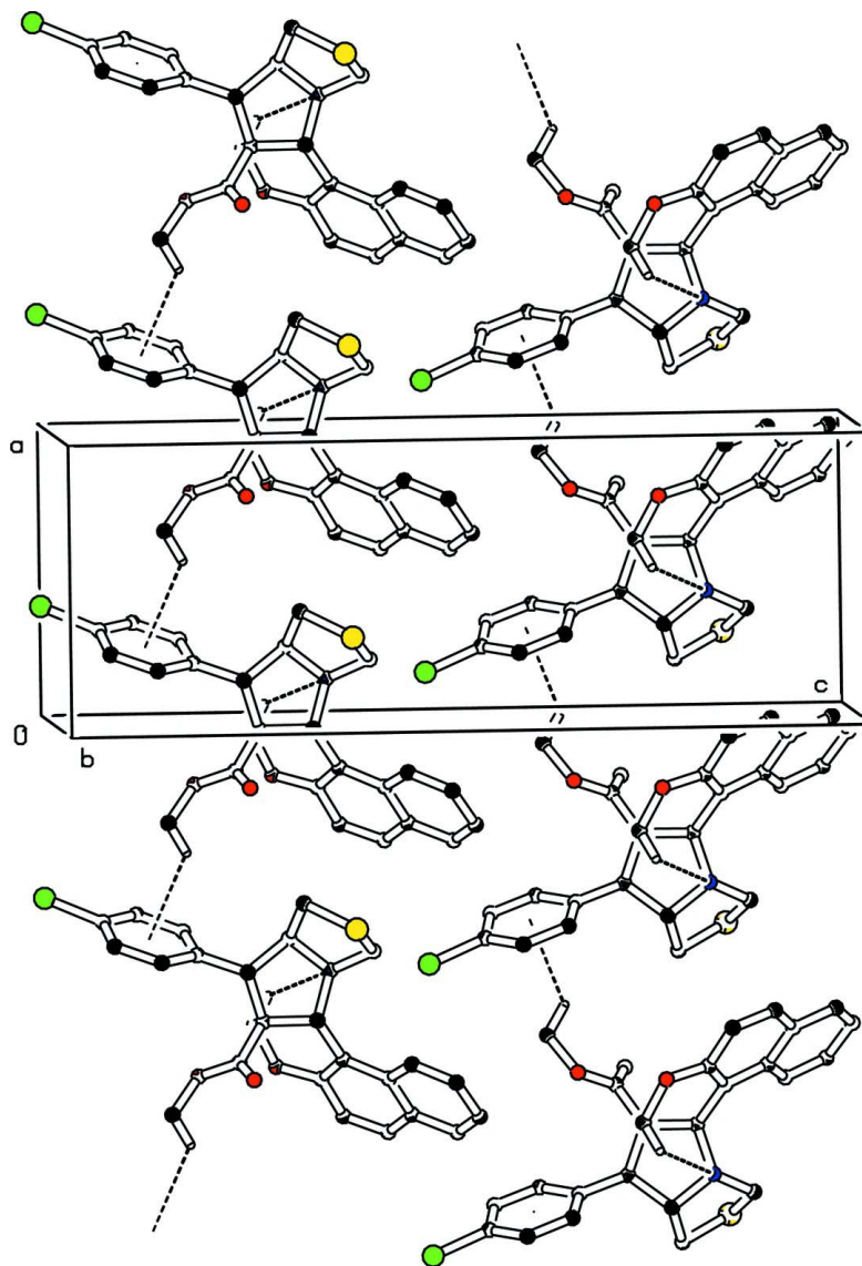
Figure 3 Molecular packing of the title compound, viewed along the b axis.
