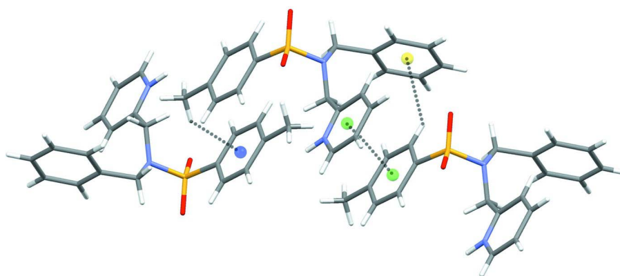
Figure 3 Crystal packing of (I) via \pi - \pi and C—H... \pi interactions, indicated as dashed lines.
