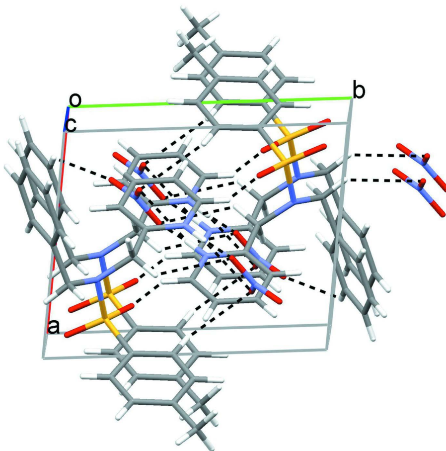
Figure 2 Crystal packing of (I). Hydrogen bonds are indicated as dashed lines.
