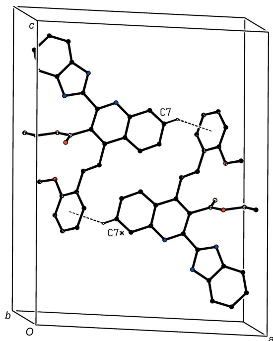
Figure 8 Part of the crystal structure of compound (IIIb), showing the formation of a cyclic centrosymmetric motif built from C–H···π hydrogen bonds and linking adjacent [010] chains. Hydrogen bonds are drawn as dashed lines and, for the sake of clarity, H atoms not involved in the motif shown have been omitted. The atom marked with an asterisk (*) is at the symmetry position (-x + 1, -y + 1, -z + 1) .
