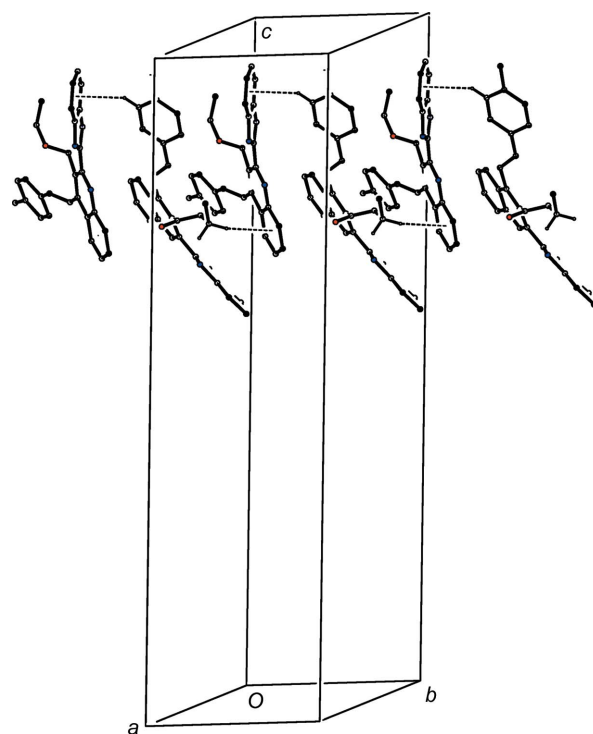
Figure 10 Part of the crystal structure of compound (IIIc), showing the formation of a chain parallel to [010] built from C–H···π hydrogen bonds (drawn as dashed lines). For the sake of clarity, the minor disorder component and the H atoms bonded to those atoms not involved in the motif shown have been omitted.
