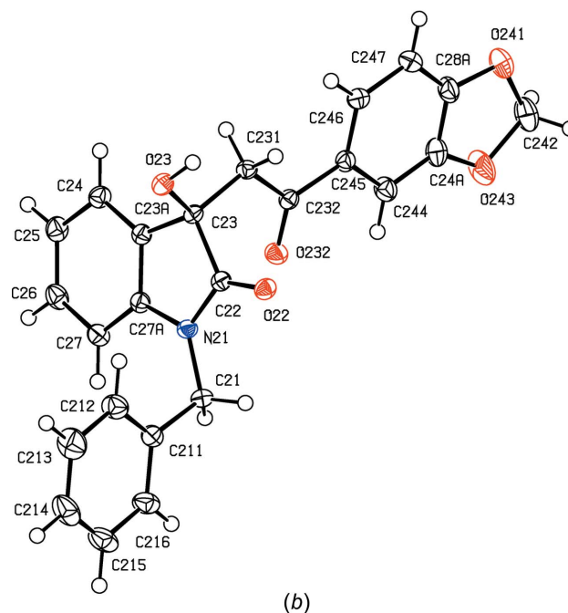
Figure 4 The R enantiomers of the two independent molecules of compound (If), showing the atom-labelling schemes for (a) molecule 1 and (b) molecule 2. Displacement ellipsoids are drawn at the 30% probability level.
