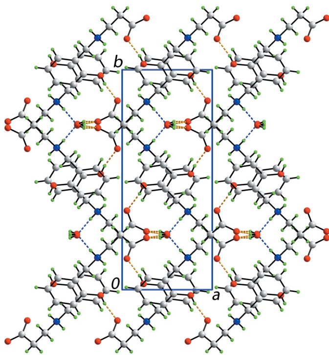
Figure 2 A view of the unit-cell contents of the title compound shown in projection down the c axis. The O—H···O and N—H···O hydrogen bonds are shown as orange and blue dashed lines, respectively.
