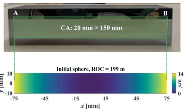
Figure 10 Initial spherical mirror with ROC = 199 m.
