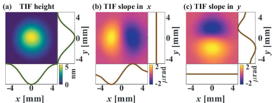
Figure 12 Height (a), slope in x (b) and slope in y (c) of the IBF TIF generated with a 5 mm diaphragm.
