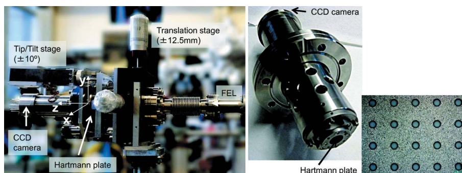
Figure 3 Left: compact Hartmann sensor. A manual operating stage allows for lateral movement in the x and y direction of \pm 12.5 mm and \pm 10^\circ tip/tilt to align the sensor to the beam. The sensor is mounted on a tripod and connected to the beamline or user experiment using a CF40 bellow. Right: inner part of the Hartmann sensor with the Hartmann plate holder. In the inset an optical microscopic image (magnification 10\times ) of part of the nickel Hartmann plate with electroformed holes is shown.
