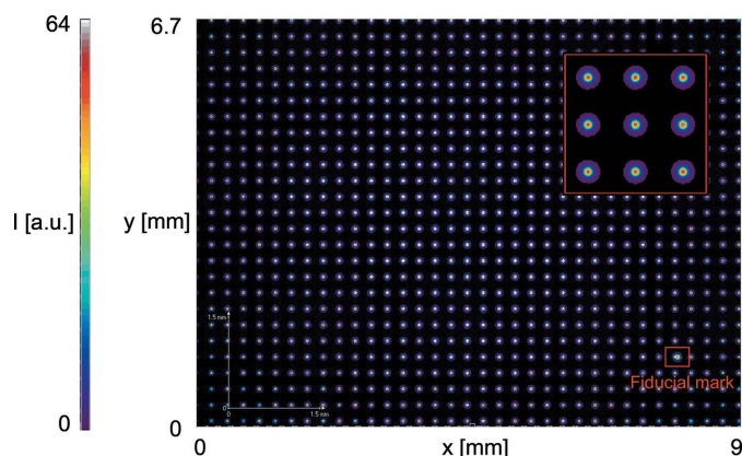
Figure 2 Compact Hartmann sensor: a reference spot pattern is created by diffraction from a 5 \mu\text{m} pinhole. For alignment purposes, one pinhole (Fiducial mark) bottom right on the Hartmann plate shows a distinct size and shape. It defines the sensor orientation and helps with the identification of individual sub-apertures.
