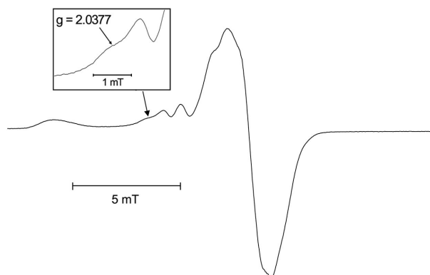
Figure 5 EPR spectrum of human insulin irradiated by \gamma -rays in air at 77 K recorded at the same temperature.
