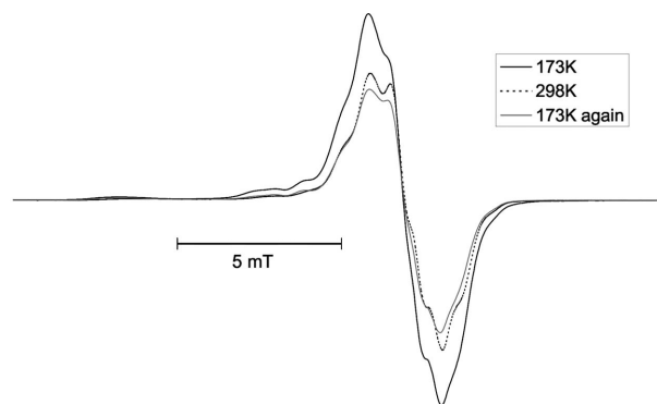
Figure 6 EPR spectra of human insulin irradiated by \gamma -rays in air at 198 K recorded at different temperature.
