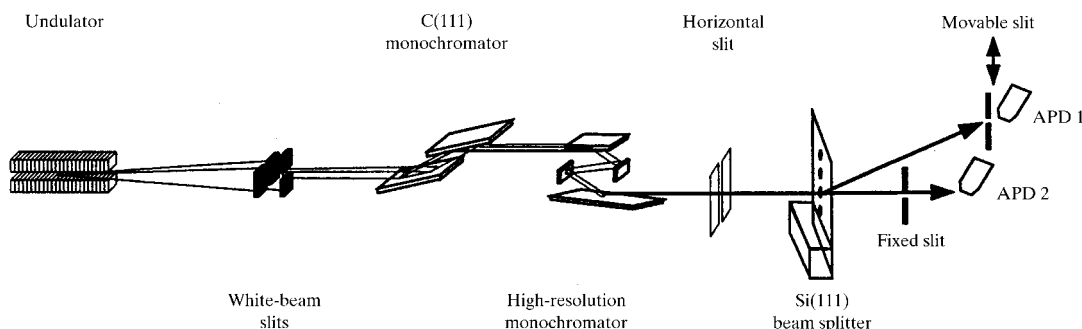
Figure 1 The experimental set-up at beamline 3-ID.
