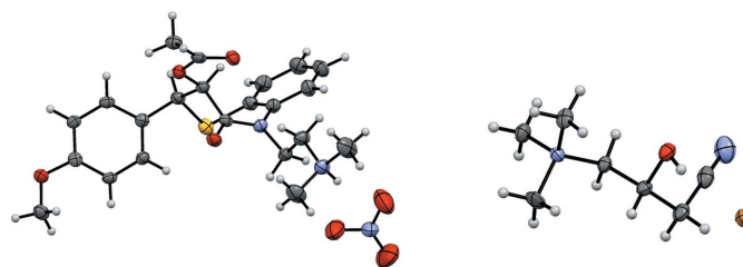
Figure 2 Left: displacement ellipsoid representation of [DiH][NO _3 ]. Right: displacement ellipsoid representation of [( - )-Car]Br. Ellipsoids are depicted at 50% probability.
