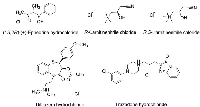
Figure 1 Chemical structures of the screened organic cations in the form of chlorides or hydrochlorides.
