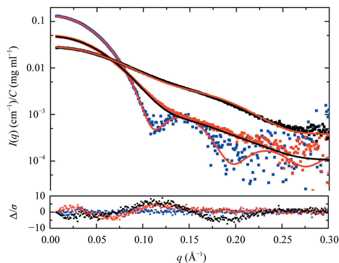
Figure 2 Crystal structure modelling results. FoXS -derived models (red and black solid lines) for GI (PDB entry 1oad, tetramer), BSA (PDB entry 4f5s, chain A ) and CaM (PDB entry 1cll with the additional N- and C-terminal residues modelled) fitted to I(q) versus q . The upper plot shows \log I(q) versus q , while the lower inset plot is the error-weighted residual difference plot \Delta/\sigma = [I_{\text{exp}}(q) - cI_{\text{mod}}(q)]/\sigma(q) versus q . The colour key for the data plots is the same as in Fig. 1.
