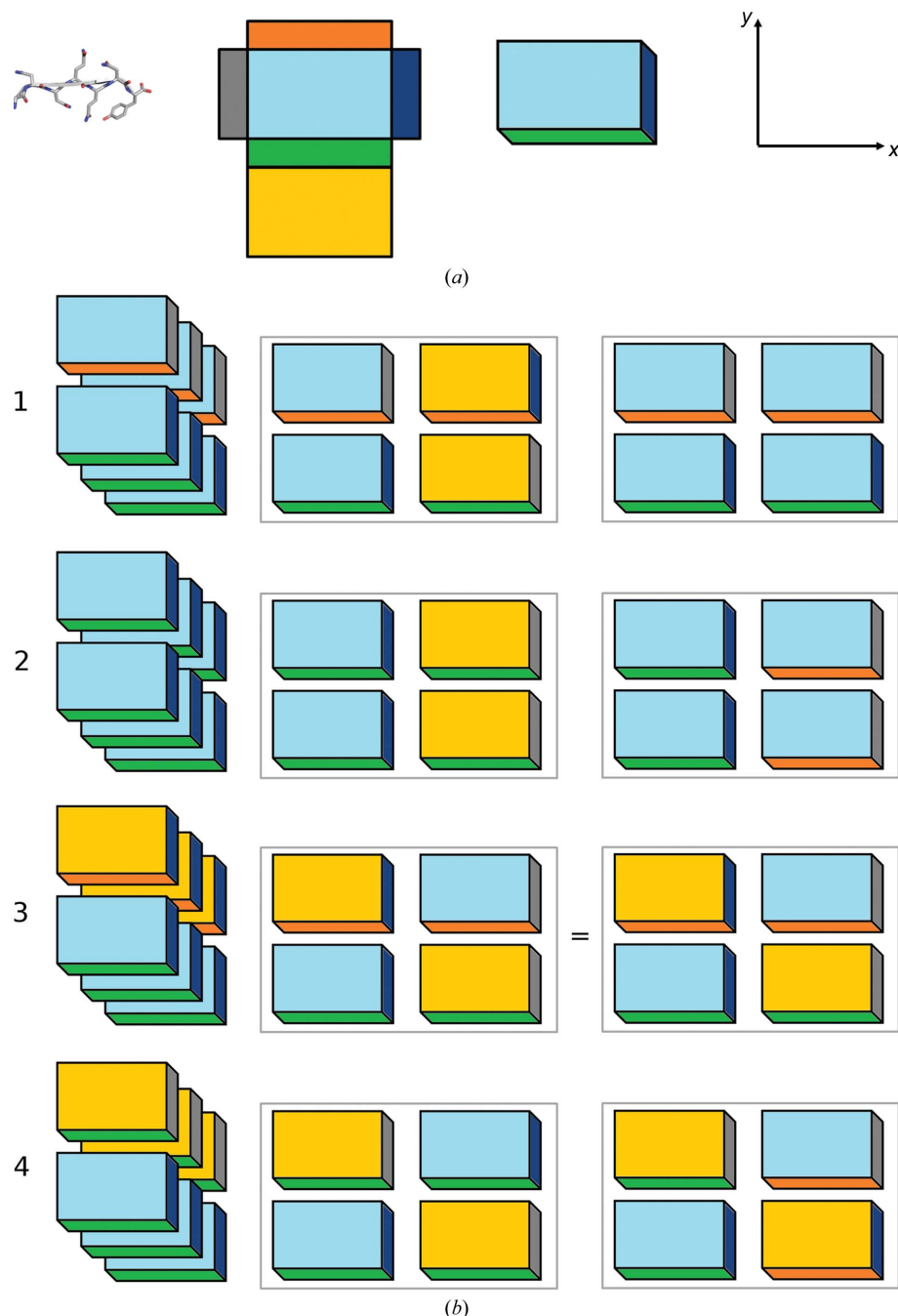
Figure 3 Packing of two-zipper motifs of class 1–4 zippers. (a) The zipper motif from the GNNQNY crystal structure (PDB entry 2omm; Sawaya et al. , 2007) is shown along with a schematic representation of a single peptide by a box (inspired by the presentation in Stroud, 2013). The different colours differentiate between C/N-termini, odd/even-residue side chains and the up/down orientation of the given \beta -sheet. (b) Left column: single zipper motifs of classes 1 to 4 for which all individual sheets are parallel. Middle column: a second zipper motif generated by rotation around a twofold axis parallel to y (perpendicular to the fibril axis). Right column: a second zipper motif generated by rotation around a twofold axis parallel to z (corresponding to the fibril long axis or spine axis).
