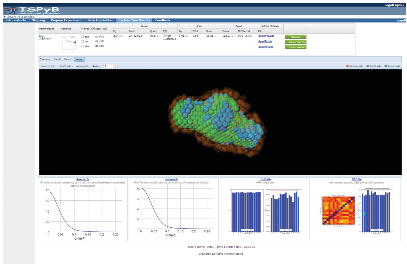
Figure 8 Ab Initio Modelling window showing the analysis results for the macromolecule and its ab initio reconstructed shape in an interactive three-dimensional rendering. Three models are shown: the average overlay ( DAMAVER , orange), the most occupied volume ( DAMFILT , green) and the DAMMIN final minimization (blue), which uses the average and filtered volume as a starting point. Close agreement between all these models indicates more robust reconstruction and thus minimal artefacts of flexibility/aggregation.
