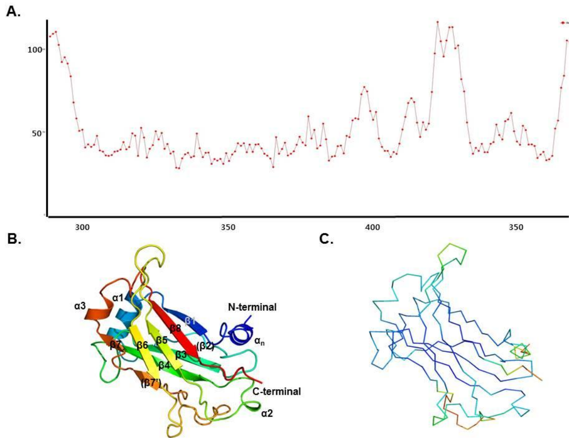
Supplementary Figure S1. A. B-factor distribution. Whole residue B-factors are plotted. The x and y axes indicate residue number and B-factor, respectively. B. The structure of TRAF4 TRAF domain. Secondary structures are shown. C. B-factor distribution on the structure. Warm and cold colors indicate high and low B-factor, respectively.
