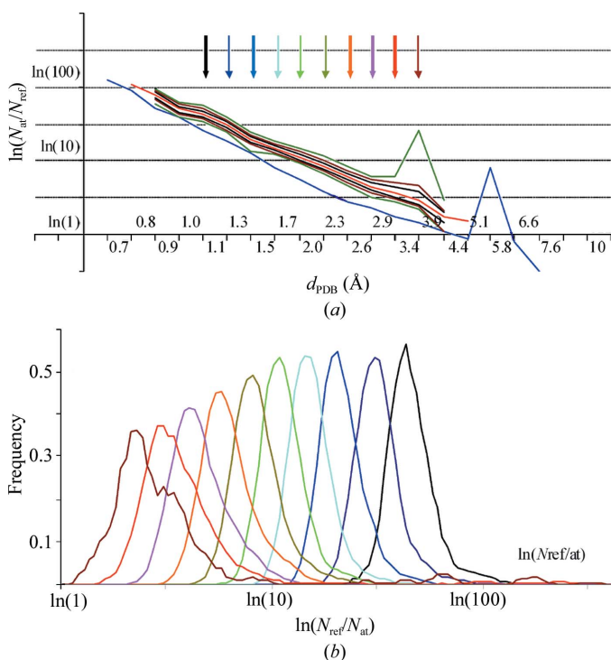
Figure 3 (a) The mode \mu(N_{\text{ref}}/N_{\text{at}}) as a function of the resolution d_{\text{PDB}} on a uniform logarithmic scale. The thick red curve shows the mode values as a function of resolution on a uniform logarithmic scale for the protein structures reported in the PDB (set 2). The thin lines show, as corridors, the distribution of the models around the mode. Each corridor contains 40% (black), 60% (brown) and 80% (dark green), respectively, of the structures in the corresponding resolution shell, half above and half below the mode. The corridors are shown at a resolution interval with a high enough number of models to calculate these values; the mode was formally calculated and is also shown for one higher resolution interval and one lower resolution interval even when the statistics there were poor. The blue line shows the minimal values for comparison (Table 1). Coloured arrows correspond to the distributions shown in (b). (b) Distribution of N_{\text{ref}}/N_{\text{at}} for several selected resolutions as indicated by coloured arrows in (a).
