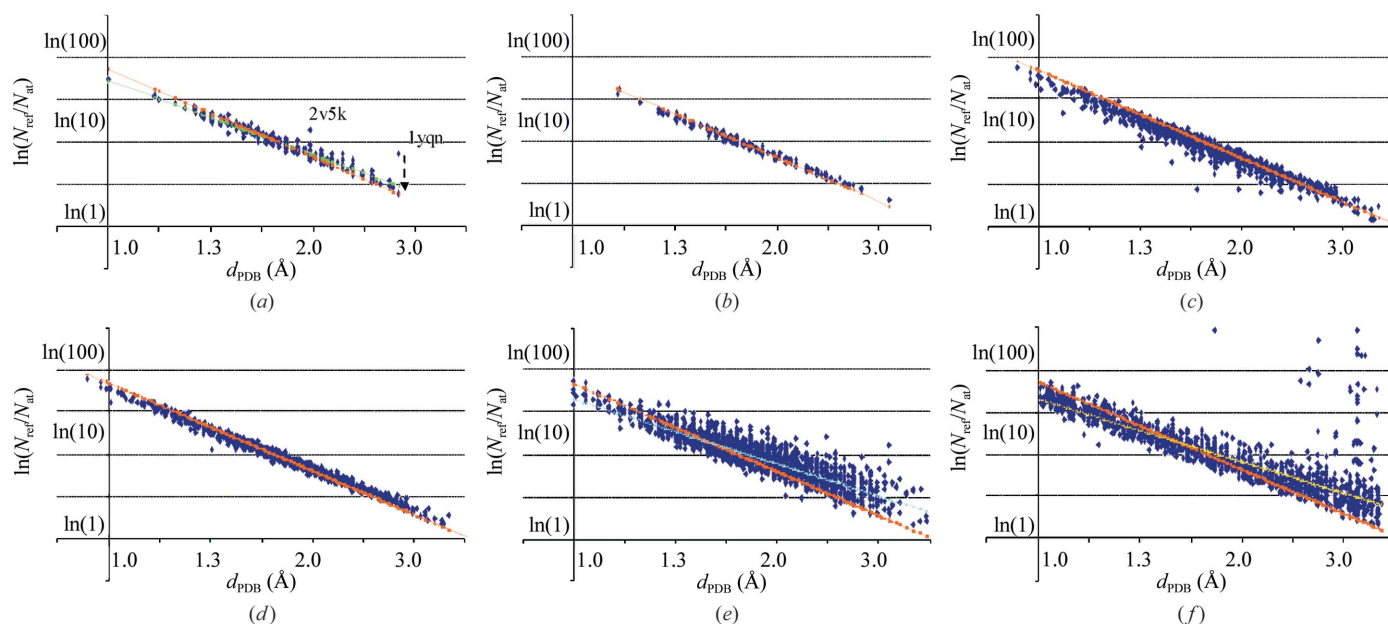
Figure 1 Distribution of the \ln(N_{\text{ref}}/N_{\text{at}}) value versus resolution d_{\text{PDB}} on a uniform logarithmic scale. (a) Structures with Matthews coefficient 2.35 < V_{\text{M}} < 2.45 \text{ \AA}^3 \text{ Da}^{-1} . V_{\text{M}} is taken from the file headers and data completeness is above 99%. The broken arrow shows the change in the ratio after a correct assignment of N_{\text{at}} for 1yqn. (b) The same as (a) but with V_{\text{M}} recalculated. (c) The same as (b) but without selection of entries by data completeness. (d) The same as (c) but with correction for data completeness. (e) All models with data completeness above 99%. (f) Random selection from the whole PDB with correction for data completeness. The orange line corresponds to theoretical values for crystals with V_{\text{M}} = 2.4 \text{ \AA}^3 \text{ Da}^{-1} . The green, blue and yellow lines show the linear approximations for (a), (e) and (f), respectively. See text for details.
