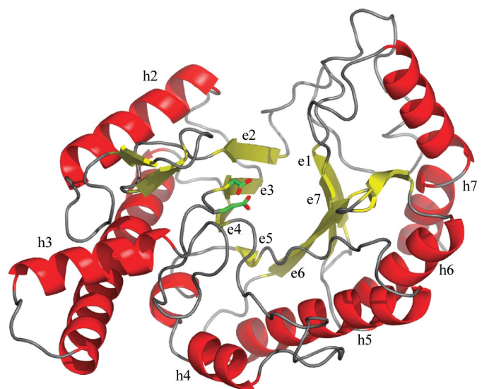
Figure 5 Overall fold of rVes v 2, including active-site residues Asp107 and Glu109. β -sheets (e1–e7) and α -helices (h2–h7) of the ( β/α ) 7 core are labelled. The assignments of the secondary-structural elements (e for extended β -strand and h for helix) in the polypeptide chain were made with the program DSSP Kabsch & Sander, 1983).
