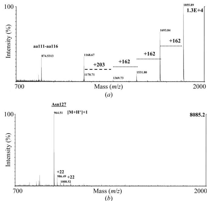
Figure 4 MALDI-TOF MS analyses of the N -glycosidic peptide from nVes v 2. Spectra of the glycopeptide, identified as amino acids 127–134 before (a) and after (b) enzymatic treatment with N -glycosidase. The masses referring to monosaccharides are included.
