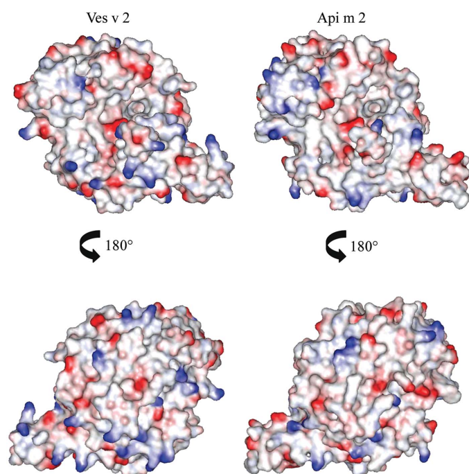
Figure 9 Surface of rVes v 2 and Api m 2 coloured by electrostatic potential (blue, positive; red, negative).
