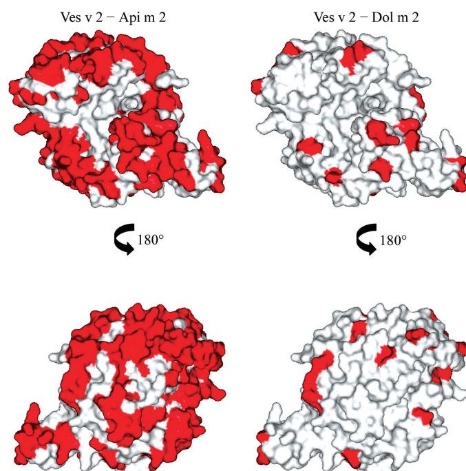
Figure 10 Solvent-accessible surface of rVes v 2 coloured by amino-acid identity to Api m 2 and Dol m 2. Identical residues are coloured white, whereas differences are shown in red.
