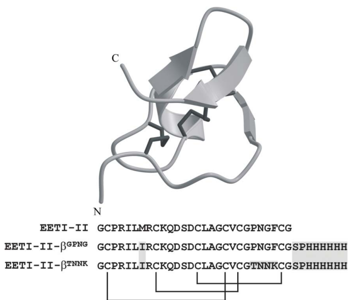
Figure 1 The cystine-knot motif in EETI-II and the sequences of the proteins investigated in this study. The sequence of EETI-II isolated from seeds of jumping cucumber E. elaterium was C-terminally extended by amino acids SPHHHHHH for affinity chromatography. The mutation M7I was introduced for purification purposes. Sequence deviations compared with the sequence of native EETI-II are highlighted in grey.
