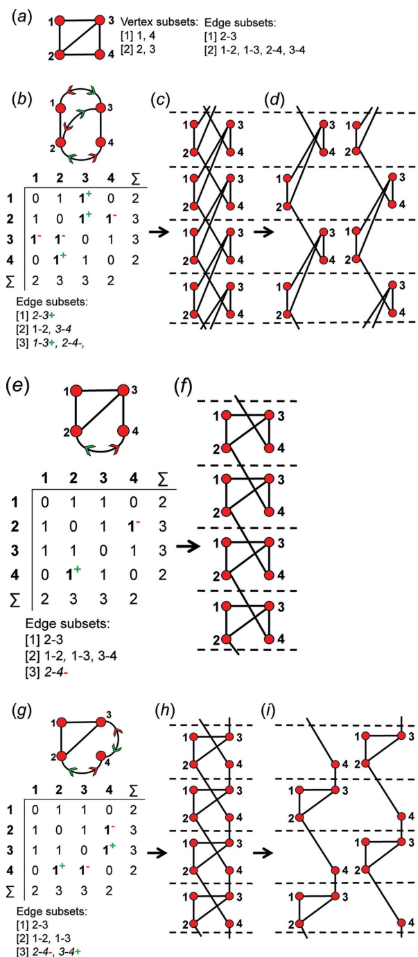
Figure 25 For vertex connectivity {}^2V_2{}^3V_2 , (a) a proto-graph [identical to that in Fig. 20(a)] and the corresponding vertex and edge subsets, (b) the directed proto-graph in which the 1–3 and 2–3 edges are assigned as wrapped in the +c direction and the 2–4 edge in the –c direction, its corresponding adjacency matrix and edge subsets, (c) the resultant chain graph, (d) an untangled version of this chain graph. (e) The directed proto-graph produced by omitting redundant unwrappings involving vertex 3 in (b), its corresponding adjacency matrix and edge subsets, and (f) the resultant chain graph which is non-isomorphic with the chain graph in (c). (g) The directed proto-graph in which the 2–4 edge is assigned as wrapped in the –c direction and the 3–4 edge is assigned as wrapped in the +c direction, its corresponding adjacency matrix and edge subsets, (h) the resultant chain graph, and (i) an untangled version of this chain graph. Note the chain graphs in (h) and (i) are isomorphic with the chain graphs in (c) and (d). Legend as in Figs. 7 and 21.
