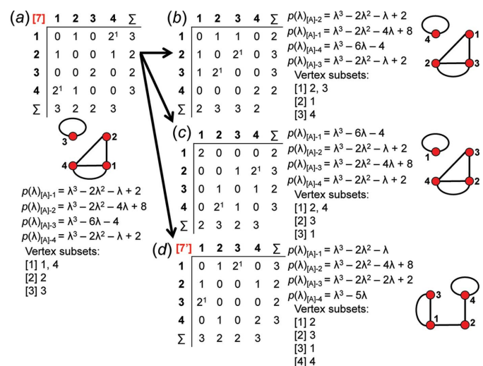
Figure 15 For vertex connectivity {}^2V_2{}^3V_2 , (a) adjacency matrix [7] for the matrix-element combination (4 × 1)(1 × 2)(2 × 2 1 ), the corresponding proto-graph, the characteristic polynomial equations of the reduced proto-graphs and the resulting vertex subsets. (b), (c), (d) Three permuted versions of this adjacency matrix and proto-graph, and the characteristic polynomial equations of the reduced adjacency matrices. The characteristic polynomial equations of the reduced adjacency matrices in (b) and (c) are identical to those in (a) (adjacency matrix [7]), confirming that the reduced proto-graphs are isomorphic. The characteristic polynomial equations for the reduced adjacency matrices derived from adjacency matrix [7'], shown in (d), are different, confirming that this proto-graph is non-isomorphic with the other proto-graphs.
