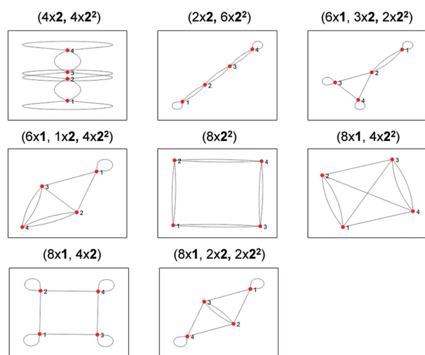
Figure 18 The MatLabR2019b output of all possible valid matrix-element combinations and corresponding non-isomorphic proto-graphs for the vertex connectivity {}^4V_4 .
