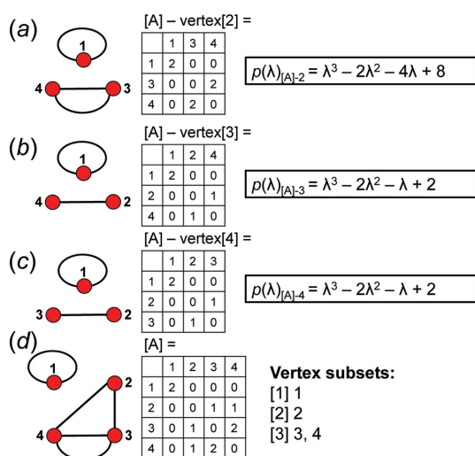
Figure 11 The reduced graphs, corresponding reduced adjacency matrices, and characteristic polynomial equations after the following vertices have been removed from the graph in Fig. 10(a): (a) vertex 2, p(\lambda)_{[A]-2} ; (b) vertex 3, p(\lambda)_{[A]-3} and (c) vertex 4, p(\lambda)_{[A]-4} . (d) The original graph, adjacency matrix and the vertex subsets determined using characteristic polynomial equations.
