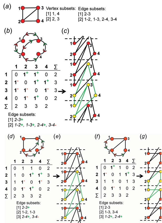
Figure 24 For vertex connectivity {}^2V_2^3V_2 , (a) a proto-graph [identical to that shown in Fig. 20(a)] and the corresponding vertex and edge subsets, (b) the directed proto-graph in which the 1–2, 1–3, 2–3 and 2–4 edges are assigned as wrapped in the +c direction and the 3–4 edge is assigned as wrapped in the -c direction, its corresponding adjacency matrix and edge subsets, and (c) the resultant chain graph. (d) The directed proto-graph produced by omitting redundant unwrappings involving vertex 1 in (b), its corresponding adjacency matrix and edge subsets, and (e) the resultant chain graph. (f) The directed proto-graph produced by omitting redundant unwrappings involving vertex 3 in (b), its corresponding adjacency matrix and edge subsets, and (g) the resultant chain graph. Note that the chain graphs in (c), (e) and (g) are isomorphic. Legend as in Figs. 7 and 21.
