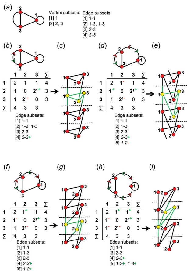
Figure 26 For vertex connectivity {}^3V_2{}^4V_1 , (a) a proto-graph for the matrix-element combination (4 \times 1)(2 \times 1)(2 \times 2^1) and its vertex and edge subsets, (b) the directed proto-graph in which the 2–3 edge is assigned as wrapped in the +c direction, its corresponding adjacency matrix and edge subsets, and (c) the resultant chain graph. (d) The directed proto-graph in which the 2–3 edge is assigned as wrapped in the +c direction and the 1–2 edge is assigned as wrapped in the -c direction, and the corresponding adjacency matrix and edge subsets, and (e) the resultant chain graph. (f) The directed proto-graph in which the 2–3 and 1–2 edges are assigned as wrapped in the +c direction, its corresponding adjacency matrix and edge subsets, and (g) the resultant chain graph. (h) The directed proto-graph in which the 2–3, 1–2 and 1–3 edges are assigned as wrapped in the +c direction, its corresponding adjacency matrix and edge subsets, and (i) the resultant chain graph. Note that the chain graphs in (e) and (i) are isomorphic with the chain graph in (c) as the unwrappings involving vertex 2 in (d) are redundant and the unwrappings involving vertex 1 in (h) are redundant. Legend as in Figs. 7 and 21.
