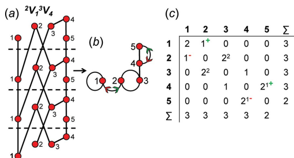
Figure 8 (a) A chain graph with vertex connectivity {}^2V_1^3V_4 , (b) the corresponding wrapped graph and (c) the corresponding adjacency matrix. Curved black lines in (b) represent wrapped edges in (a); green and red arrows in (b) and matrix-element superscripts in (c) indicate the number and direction of wrapped edges. Note that it is not necessary to indicate the direction of the wrapped edges linking vertices 2 and 3. Dashed black lines show the repeat units of each chain graph.
