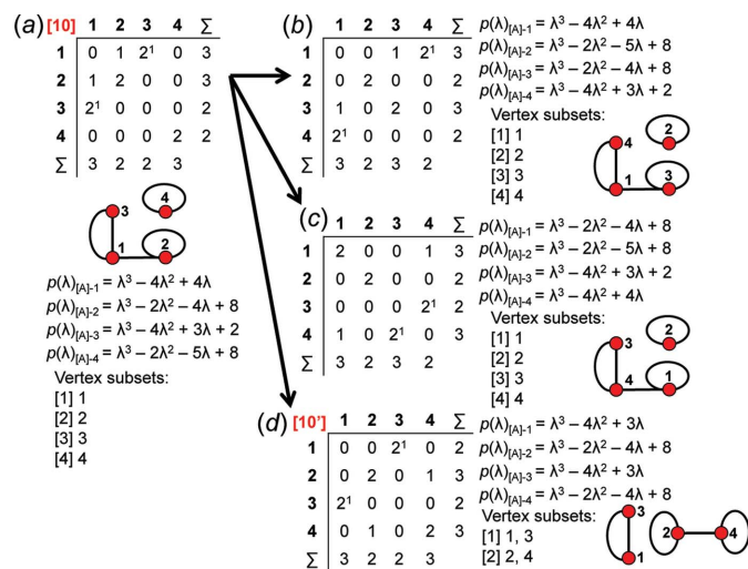
Figure 16 For vertex connectivity {}^2V_2{}^3V_2 , (a) adjacency matrix [10] for the matrix-element combination (2 \times 1)(2 \times 2)(2 \times 2^1) , the corresponding proto-graph, the characteristic polynomial equations of the reduced proto-graphs and the resulting vertex subsets. (b), (c), (d) Three permuted versions of this adjacency matrix and proto-graph, and the characteristic polynomial equations of the reduced adjacency matrices. The characteristic polynomial equations of the reduced adjacency matrices in (b) and (c) are identical to those in (a) (adjacency matrix [10]), confirming that these proto-graphs are isomorphic. The characteristic polynomial equations for the reduced adjacency matrices derived from adjacency matrix [10'], shown in (d), are different, confirming that this proto-graph is non-isomorphic with the proto-graphs in (b) and (c).
