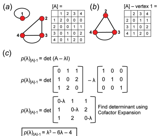
Figure 10 (a) A graph with vertex connectivity {}^2V_2{}^3V_2 and its corresponding adjacency matrix ( [A] ), (b) the reduced graph produced by removing vertex 1 from the graph in (a) and the corresponding reduced adjacency matrix ( [A]-1 ), and (c) the characteristic polynomial equation for the reduced adjacency matrix in (b): [p(\lambda)_{([A]-1)}] .
