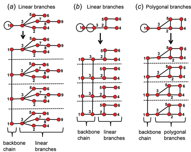
Figure 27 (a) A proto-graph and corresponding chain graph with vertex connectivity {}^1V_3{}^2V_4{}^3V_1{}^4V_1 in which edges 3–5, 3–2, 3–7, 2–4, 5–6, 7–8 and 8–9 and vertices 2 to 9 form linear branches, and edge 1–1 and vertex 1 form the backbone chain. (b) A proto-graph and corresponding chain graph with vertex connectivity {}^1V_2{}^2V_1{}^3V_2{}^4V_1 in which edges 3–2, 2–4, 2–5 and 5–6 and vertices 2, 4, 5 and 6 form linear branches and edges 1–1, 3–3 and 1–3 and vertices 1 and 3 form the backbone chain. (c) A proto-graph and corresponding chain graph with vertex connectivity {}^2V_2{}^3V_4 in which edges 3–2, 3–5, 2–5, 2–4, 5–6 and 4–6 and vertices 2 to 6 form polygonal branches, and edges 1–1 and vertex 1 form the backbone chain. Legend as in Fig. 7.
