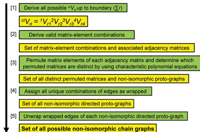
Figure 30 A flow chart of the overall method to derive all non-isomorphic chain graphs from the complete set of possible vertex connectivities {}^1V_{r1}{}^2V_{r2}{}^3V_{r3}{}^4V_{r4} . Green boxes denote actions and yellow boxes denote the products.
