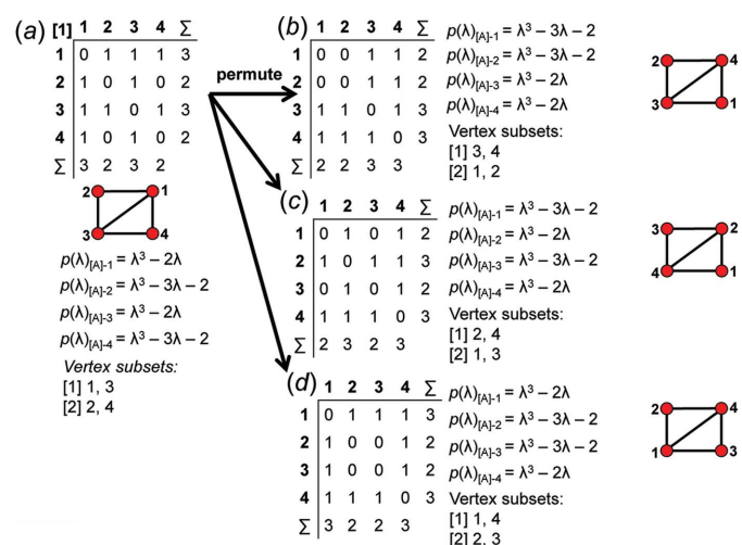
Figure 14 For vertex connectivity {}^2V_2{}^3V_2 , (a) the adjacency matrix [1] for the matrix-element combination (10 × 1), the corresponding proto-graph, the characteristic polynomial equations of the reduced proto-graphs and the resulting vertex subsets; (b), (c) and (d) three permuted versions of this adjacency matrix and proto-graph. The characteristic polynomial equations of the reduced adjacency matrices are identical, confirming that these adjacency matrices correspond to isomorphic proto-graphs.
