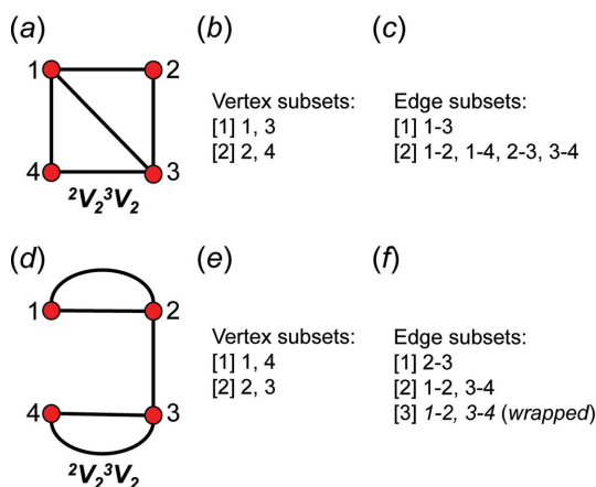
Figure 17 For vertex connectivity {}^2V_2{}^3V_2 , (a) the proto-graph for the matrix-element combination (10 \times 1) , (b) the corresponding vertex subsets, (c) the corresponding edge subsets. (d) The proto-graph for the matrix-element combination (2 \times 1)(4 \times 2^1) , (e) the corresponding vertex subsets, (f) the corresponding edge subsets.
