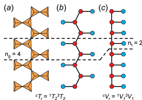
Figure 4 (a) Tetrahedron, (b) ball-and-stick and (c) graphical representations of the chain in astrophyllite-supergrupp minerals viewed orthogonally to the c axis. Each tetrahedron in (a) is represented by a point (ball) in (b) and a vertex in (c), and all linkages between tetrahedra in (a) are represented by lines (sticks) in (b) and edges in (c) that connect each ball or vertex. Red and blue balls (points) represent 3- and 1-connected vertices, respectively. Dashed black lines show the {}^1T_2{}^3T_2 geometrical repeat unit ( n_g ) in (a) and (b), and the {}^1V_1{}^3V_1 topological repeat unit ( n_t ) in (c).
