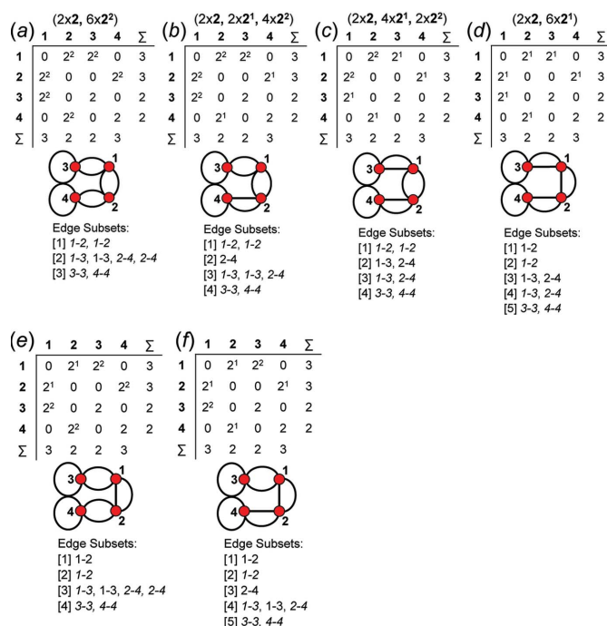
Figure 19 For vertex connectivity {}^4V_4 , the adjacency matrix, corresponding proto-graph and edge subsets for the matrix-element combinations (a) (2 \times 2)(6 \times 2^2) , (b) (2 \times 2)(2 \times 2^1)(4 \times 2^2) , (c) (2 \times 2)(4 \times 2^1)(2 \times 2^2) and (d) (2 \times 2)(6 \times 2^1) . The matrix-element combinations (2 \times 2)(2 \times 2^1)(4 \times 2^2) and (2 \times 2)(4 \times 2^1)(2 \times 2^2) correspond to a second distinct matrix and non-isomorphic proto-graph shown in (e) and (f), respectively. The adjacency matrices and corresponding proto-graphs in (b)–(f) are not produced by the MatLabR2019b code and must be derived manually. In edge subsets, wrapped edges are italicized.
