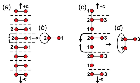
Figure 2 (a) An infinite chain graph with vertices of degree 1 and 3, in which repeat units are separated by dashed lines and edge 2–2 extends outside the repeat unit; (b) a finite wrapped graph in which edges that extend outside the repeat unit in (a) are wrapped to form a loop at vertex 2; (c) an infinite chain graph with vertices of degree 1, 2 and 3; (d) a finite wrapped graph in which edges that extend outside the repeat unit in (c) are wrapped to form a curved edge between vertices 1 and 2. Straight black arrows indicate the infinite extension of chain graphs in the +c and -c directions. Curved black arrows in (a) and (c) indicate how edges are wrapped in (b) and (d), and curved black lines represent wrapped edges in (b) and (d). Dashed black lines show the repeat units of each chain graph.
