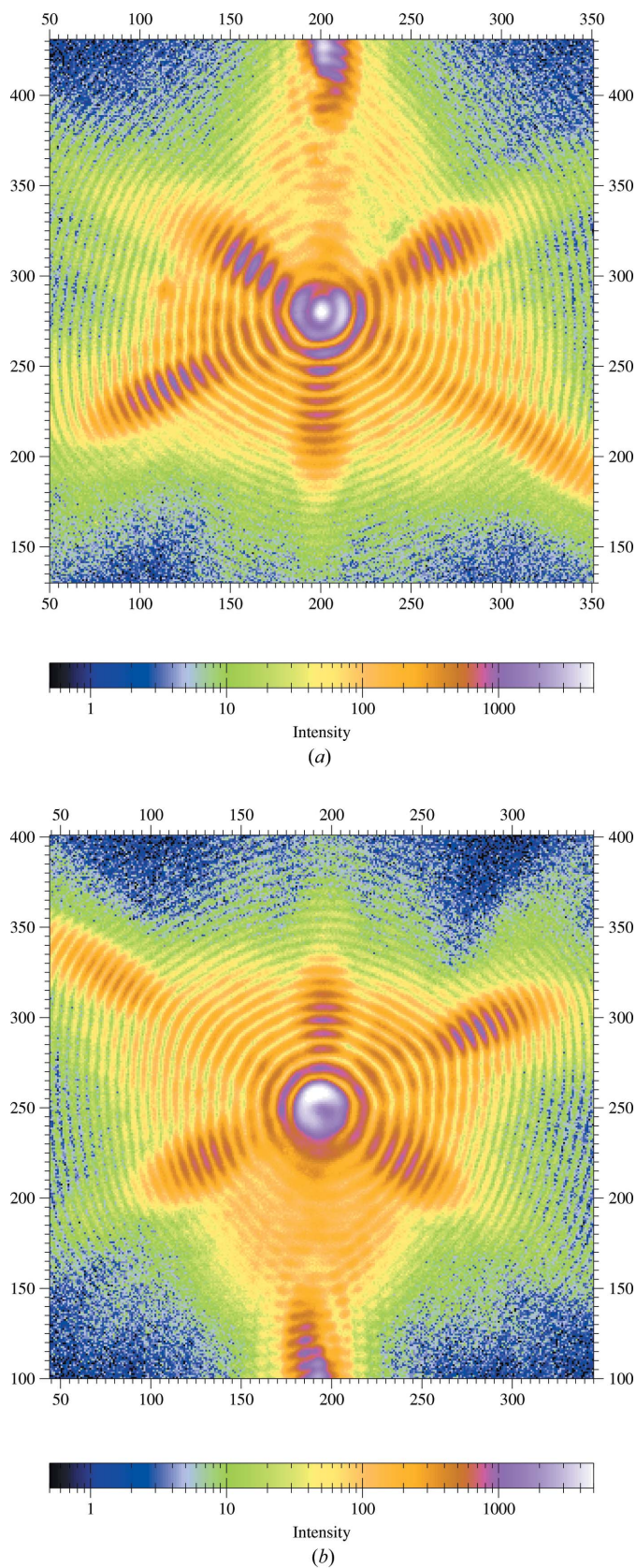
Figure 17 Diffraction from a 1 μm gold crystal measured on both sides of the center of a (111) Bragg peak, showing the high-precision central symmetry of the scattering: λ = 1.55 Å, sample-to-detector distance 0.87 m, pixel size 22 μm. Results from ID01 at the ESRF.
