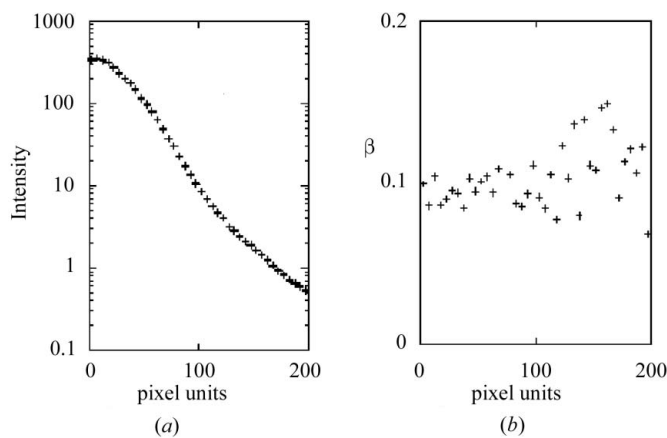
Figure 10 Angular average (log scales) (a) of the intensities of Fig. 9 over a 5 pixels ring and the corresponding estimated coherence \beta (b). Pixel units are distances to the central peak in Fig. 9, i.e. 4.4 \times 10^{-5} \text{ \AA}^{-1} per pixel.
