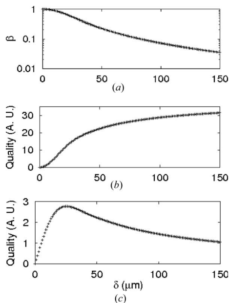
Figure 12 Typical dependence of the speckle contrast \beta versus the detector aperture \delta (a), the variations of the SNR (or quality, in arbitrary units) for a point detector (b) and with \delta as the CCD pixel size (c). Curves (b) and (c) cannot be compared. In the case of an area detector, the 22 \mu\text{m} pixel size, at this 2 m distance, is an optimum, and one should not bin pixels of the CCD.
