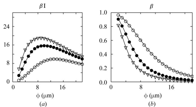
Figure 13 Calculated quality factor (SNR, arbitrary units) (a) and the corresponding speckle contrast \beta (b) for the set-up of Fig. 11: \phi_1 = 300 \mu\text{m} (triangles), 200 \mu\text{m} (closed circles) and 100 \mu\text{m} (open circles).
