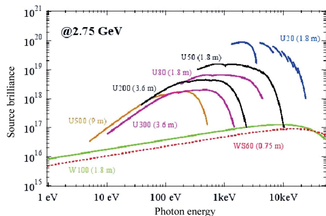
Figure 3 Estimates of brilliance of various sources for the Soleil synchrotron (France). Brilliance ( \mathcal{B} ) units are photons ( \text{s} \text{mm}^2 \text{mrad}^2 0.1\% \text{bandwidth} ) ^{-1} .
