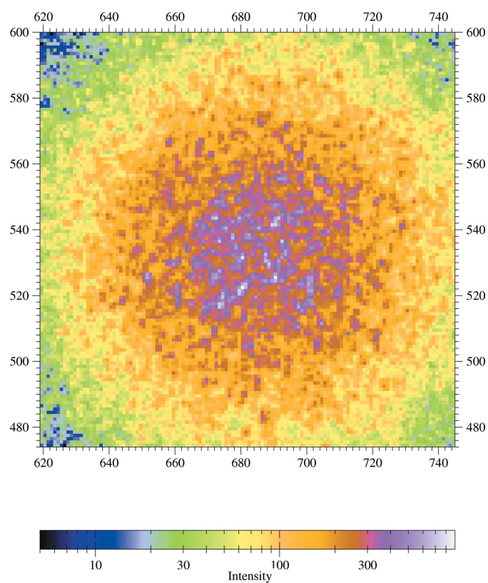
Figure 9 Diffraction from an ordered AuAgZn 2 alloy at the (\frac{1}{2}\frac{1}{2}\frac{1}{2}) Bragg superstructure position. \lambda = 1.58 \text{ \AA} , 12 \mu\text{m}^2 slits, detector with 22 \mu\text{m} pixels at 2 m (unpublished results from the ID10 beamline of ESRF).
