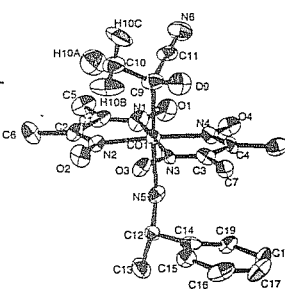
Fig. 1. Molecular structure
