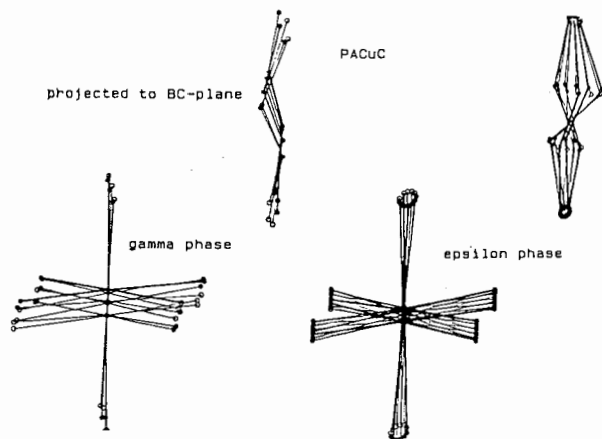
Figure 1 Loci of modulated atoms which are pulled back to the original unit cell of (\text{C}_3\text{H}_7\text{NH}_3)_2\text{CuCl}_4 in the \gamma (Fig.1) and \epsilon (Fig.2) phases, looking from the a -axis.
