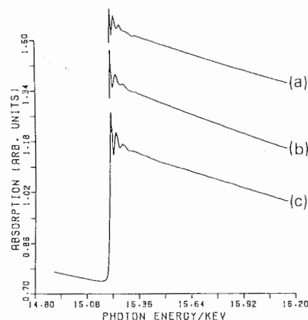
Fig. 1. Rubidium K-edge X-ray absorption spectra of (a) superconducting \text{Rb}_3\text{C}_{60} , (b) air exposed \text{Rb}_3\text{C}_{60} and (c) \text{RbHTr} at room temperature.
