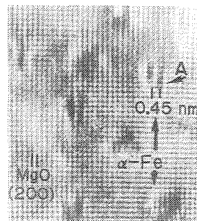
Fig.2 Electron micrograph of as-grown composite film
