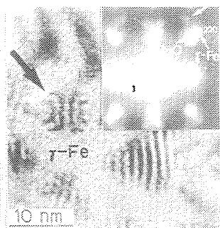
Fig.3 Electron micrograph and microdiffraction pattern of \gamma -iron crystallite after heat-treatment.
