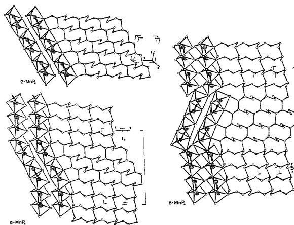
Fig. 2. Crystal structures of three modifications of MnP_4 .
