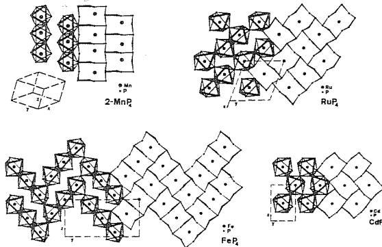
Fig. 1. Crystal structures of 2- MnP_4 , RuP_4 , \alpha - FeP_4 , and CdP_4 .
