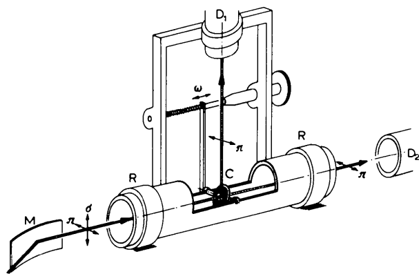
Fig. 3. Device for measurement of the polarization ratio, K ; in the figure set for \pi polarization. The structures are attached to a hollow cylinder, supported by rings R so as to allow a 90^\circ rotation to measure the \sigma polarization. The axis of the cylinder is aligned to coincide with the incident beam from monochromator M . C is a perfect crystal or a powder sample, and D_1 and D_2 are the detector positions in reflection and transmission, respectively. The \omega scan is arranged with a micrometer screw driven by a synchronous motor; in the powder measurement the motor spins the specimen by chord transmission.
